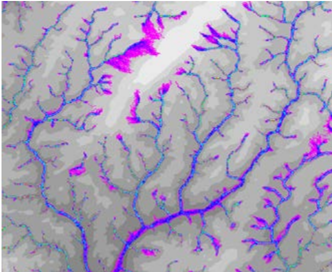
Figure 18. Number of hits for a cell being part of the drainage network for 50 noised digital elevation maps. From purple via dark blue to light blue the number of hits grows.
