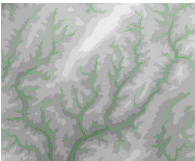
Figure 16. Drainage pattern of the part of the Prüm as the results of traditional GIS hydrological analysis (see also part 1)
