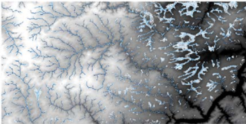
Figure 19. Results of the Digital elevation flow path approach for the Elsbach catchment.
