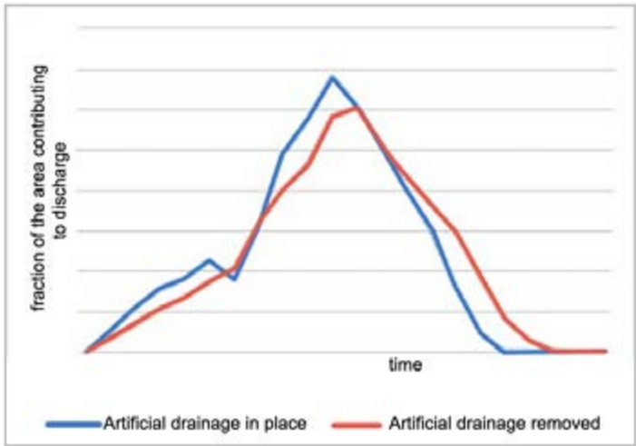
Figure 20. Synthetic discharge hydrograph based on the travel time in the Elsbach catchment for situations with (red line) and without (blue line) sponge restoration.
