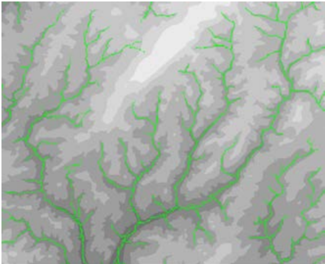
Figure 17. Drainage pattern of the part of the Prüm as the results of the newly developed Digital elevation flow path approach.
