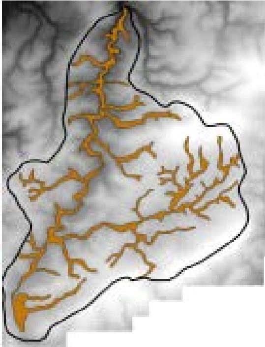
Figure 21. Results of the Digital elevation flow path approach for the Ruwer catchment.
