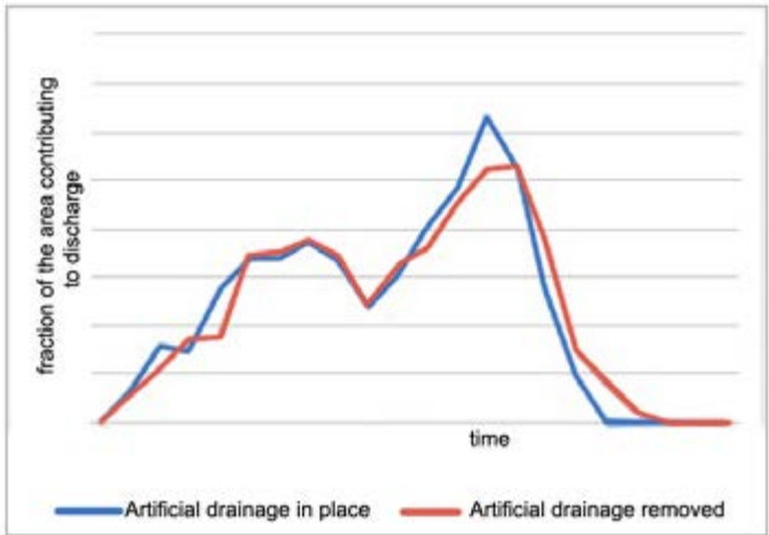
Figure 22. Synthetic discharge hydrograph based on the travel time in the Ruwer catchment for situations with (red line) and without (blue line) sponge restoration.
